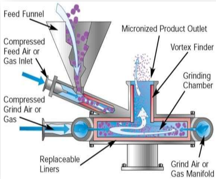
FLUID ENERGY MILL
