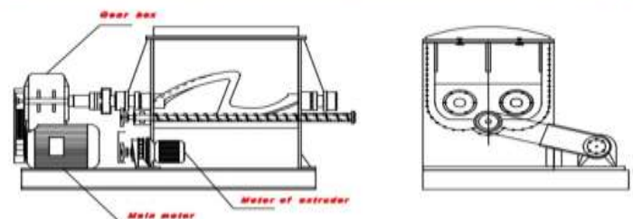
SIGMA BLADE MIXER
