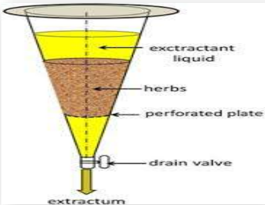
PERCOLATOR
