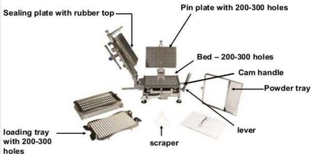
CAPSULE FILLING MACHINE (MANUAL)
