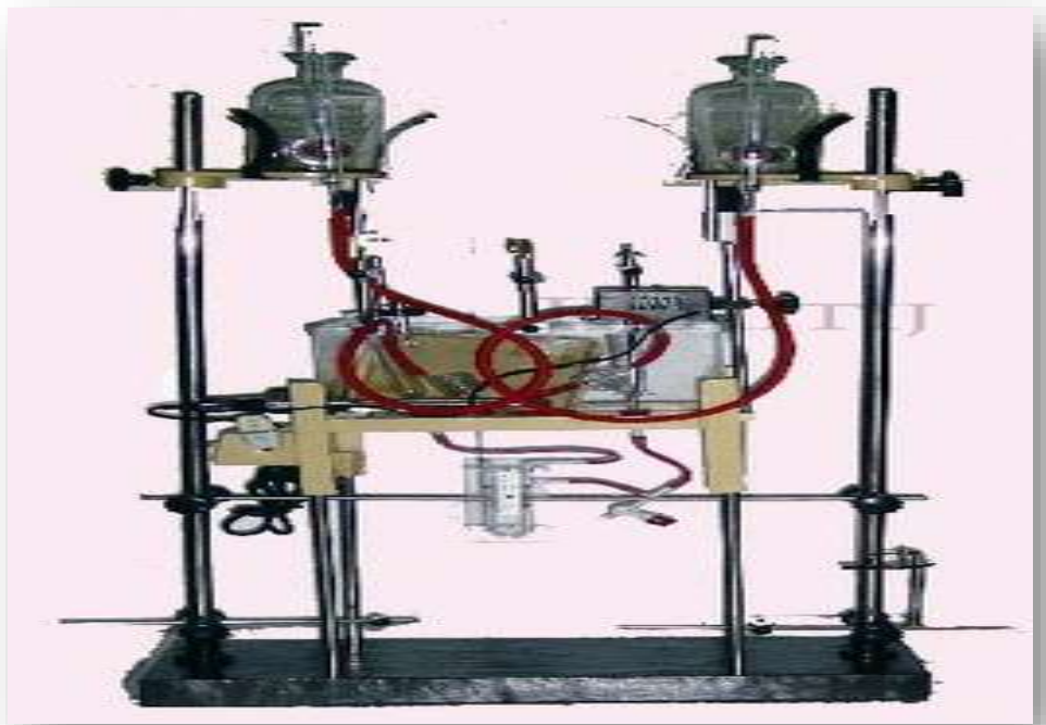
LAGENDROFF ASSEMBLY
