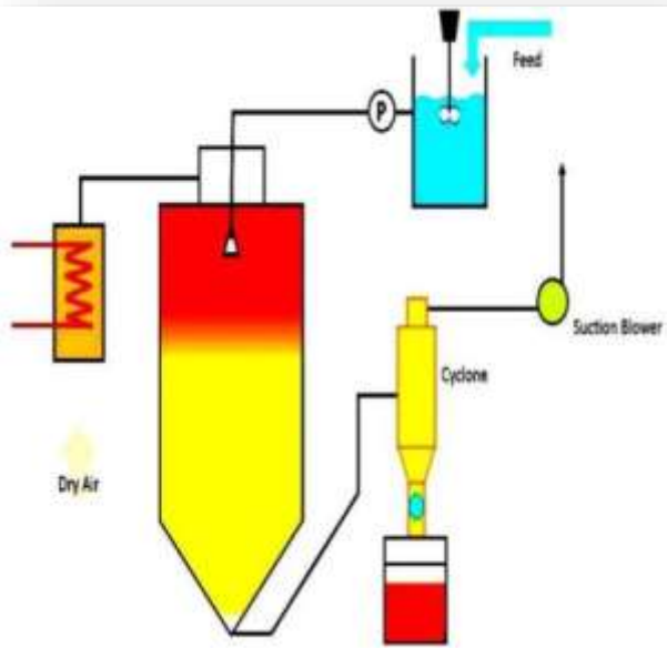
SPRAY DRYER
