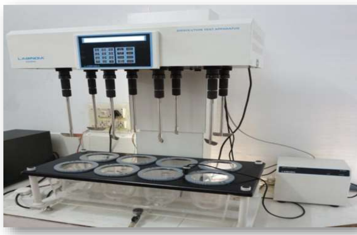
DISSOLUTION TESTING APPARATUS, ROTATING PADDLE (USP TYPE II)
