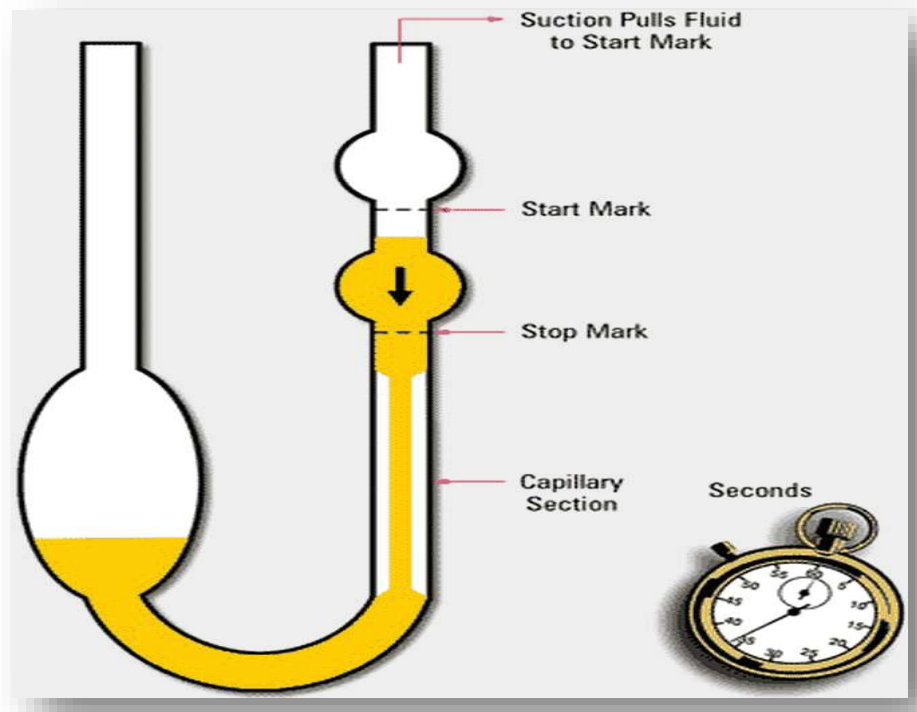
OSTWALD'S VISCOMETER
