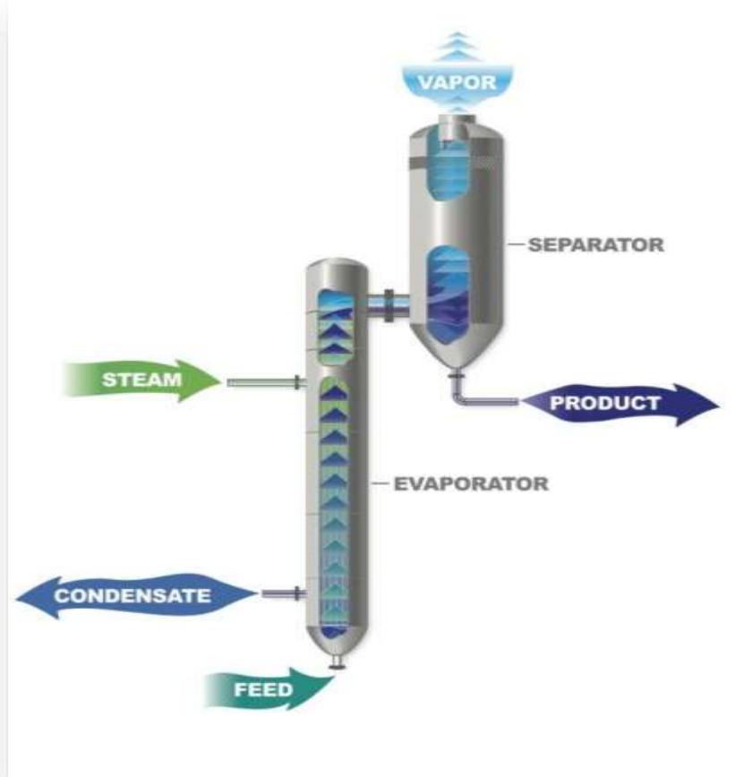
FILM TYPE EVAPORATORS
