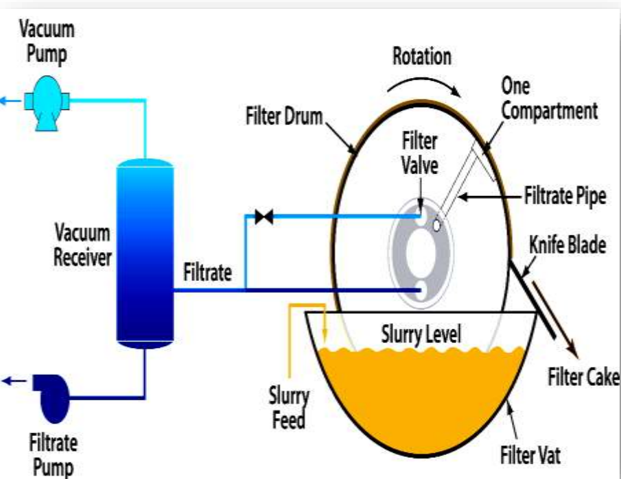
ROTARY DRUM FILTER
