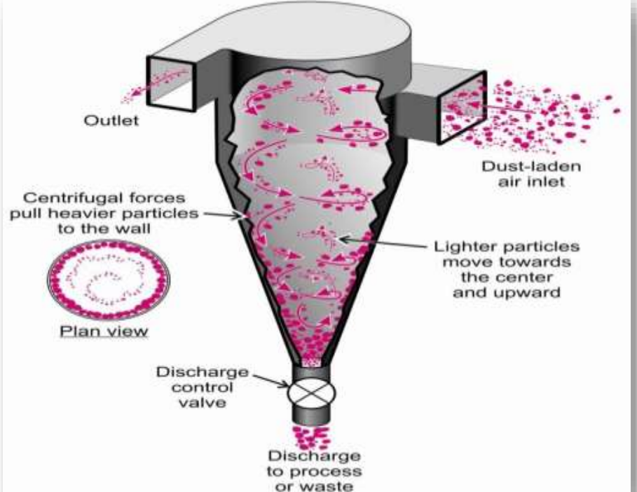
CYCLONE SEPARATOR
