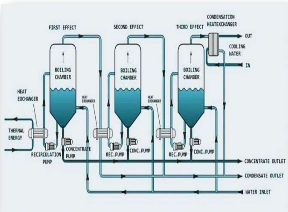
MULTIPLE EFFECT EVAPORATOR
